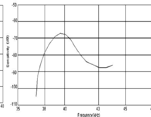
SPL-Frequency Characteristics
